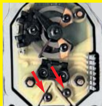
Deposits on the surfaces of copper parts (black oxidized) in the half-differential short-circuiting ring due to aggressive components in FAME.
